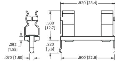
Mounting Detail
