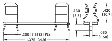
Mounting Detail
