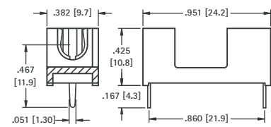
Mounting Detail
